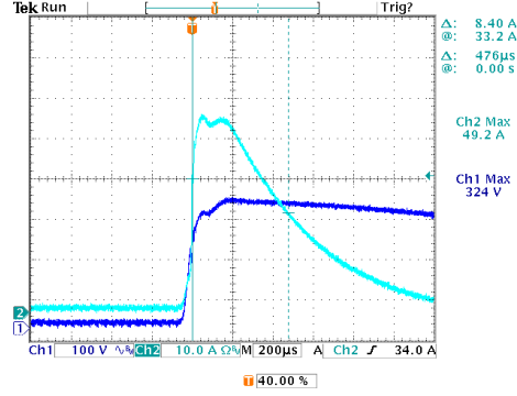
CH2: Input current CH1: AC Input Voltage
