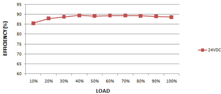
EFFICIENCY vs LOAD
